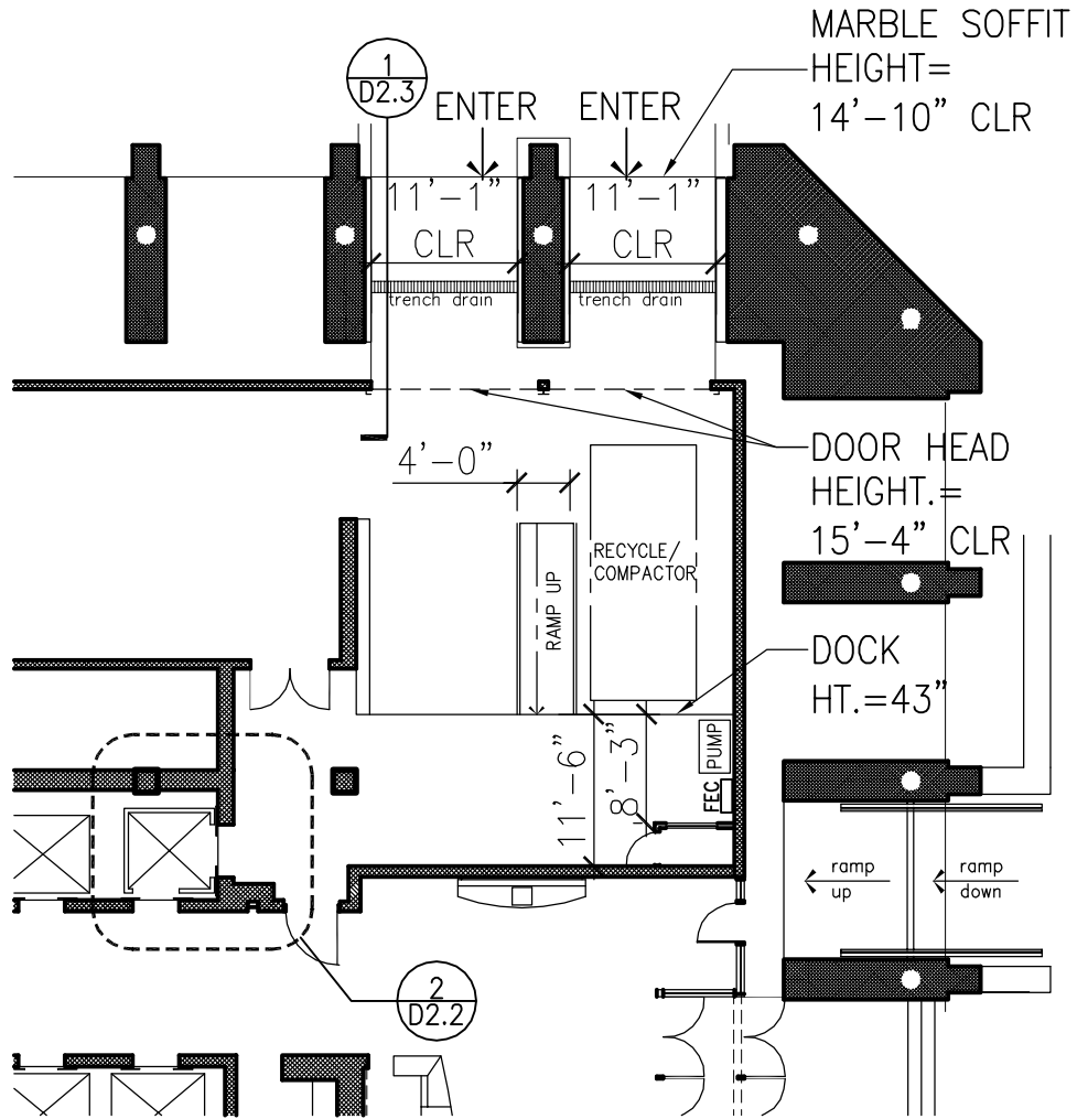
1 PARTIAL FIRST FLOOR PLAN
