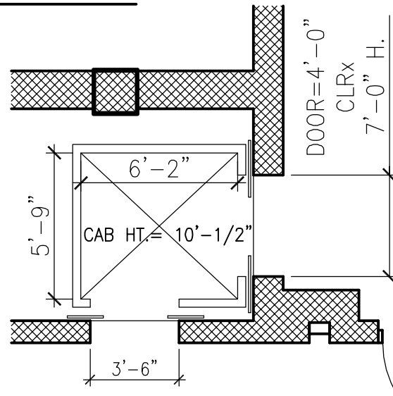
2 ENLARGED FREIGHT ELEVATOR PLAN
