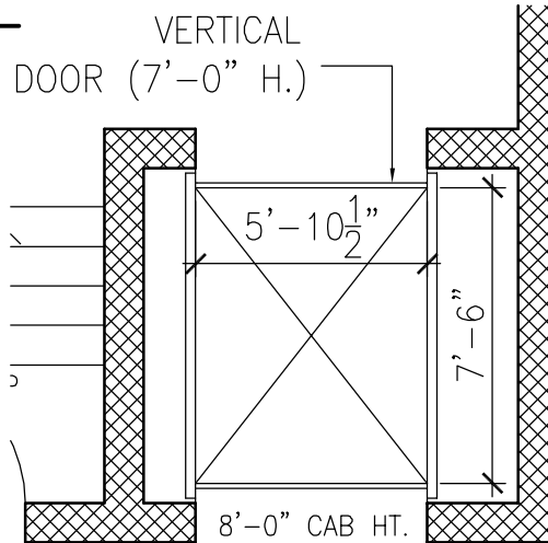
2 ENLARGED FREIGHT ELEVATOR PLAN
