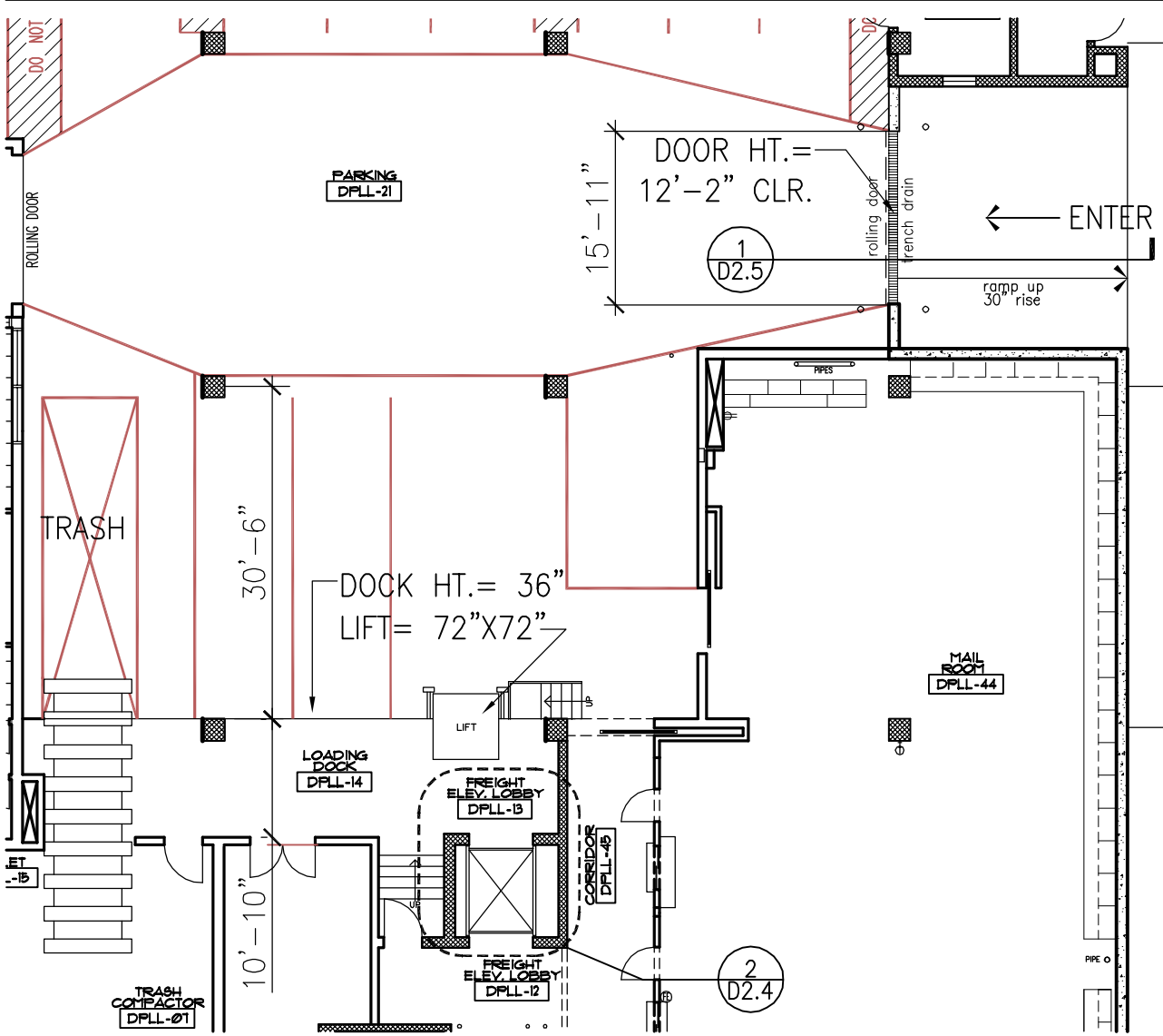
1 PARTIAL LOWER LEVEL FLOOR PLAN
